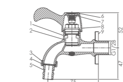
Model No: QP15-1A single way faucet for washing machine
